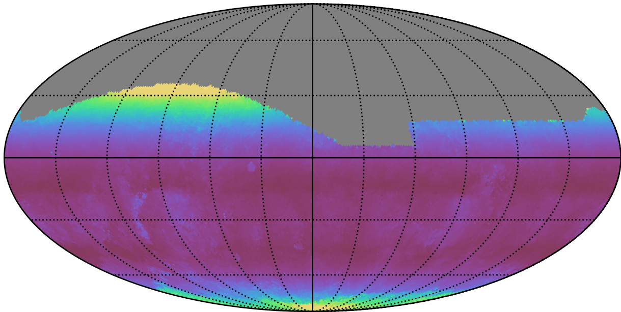
extra_ss_neo7_v3.4_10yrs All sky g band: Median airmass
