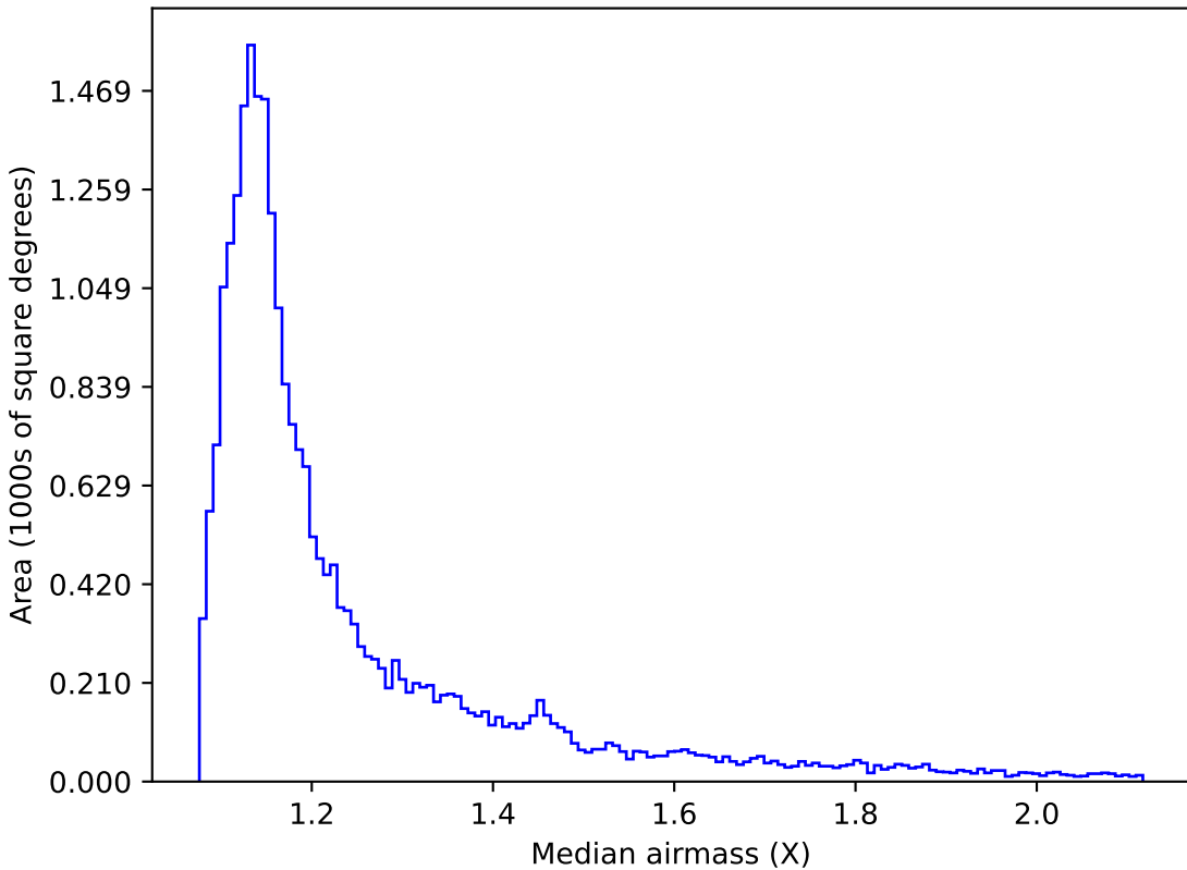
extra_ss_neo7_v3.4_10yrs All sky g band: Median airmass
