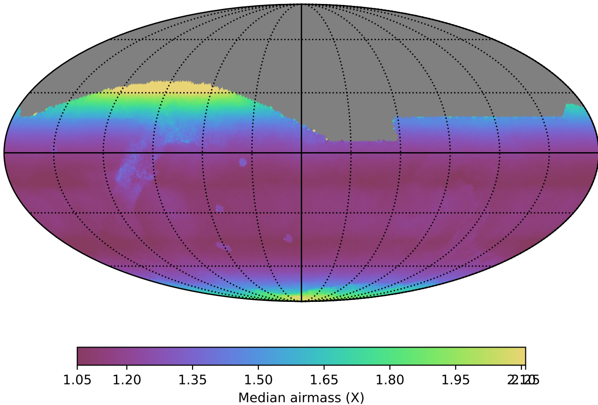
extra_ss_neo7_v3.4_10yrs All sky all bands: Median airmass
