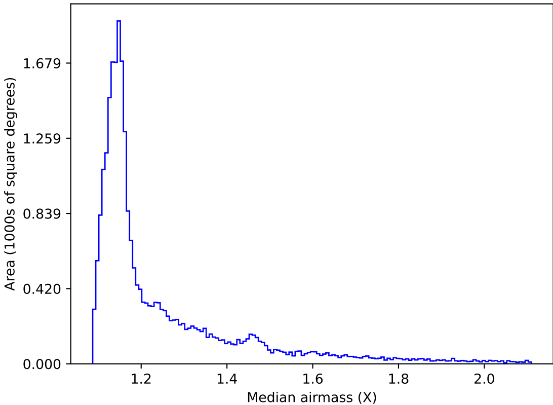
extra_ss_neo7_v3.4_10yrs All sky all bands: Median airmass
