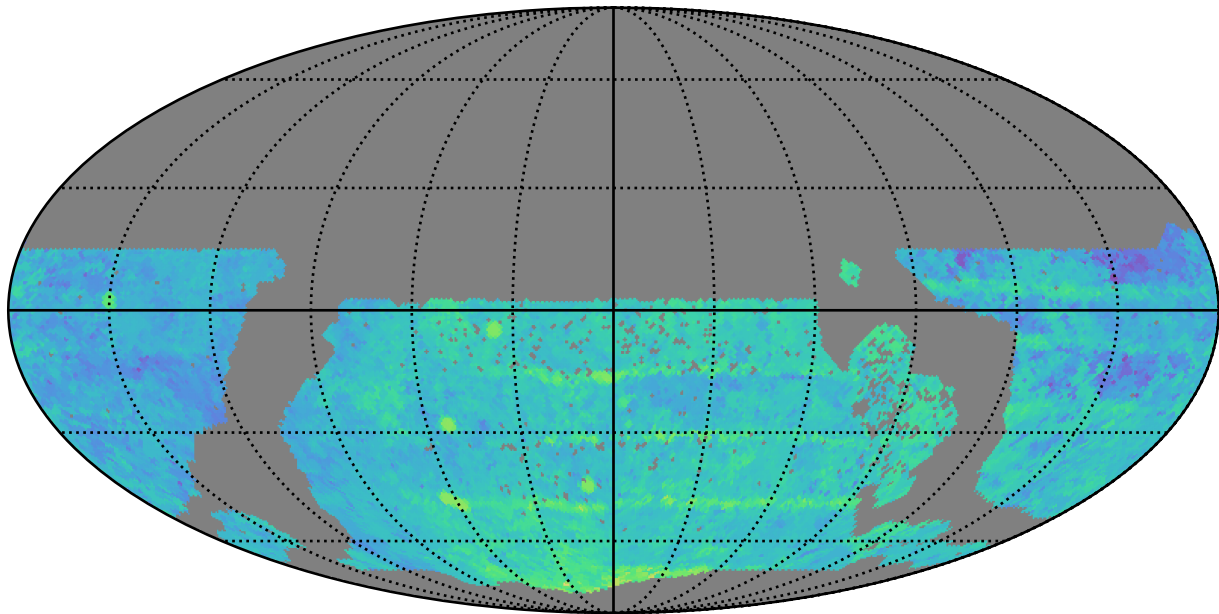
extra_ss_neo7_v3.4_10yrs WFD z band: Median Season Length
