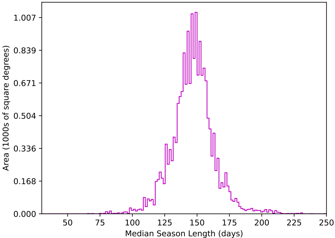
extra_ss_neo7_v3.4_10yrs WFD z band: Median Season Length
