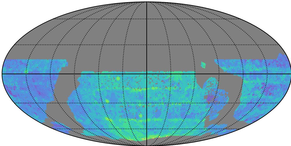
extra_ss_neo7_v3.4_10yrs WFD y band: Median Season Length
