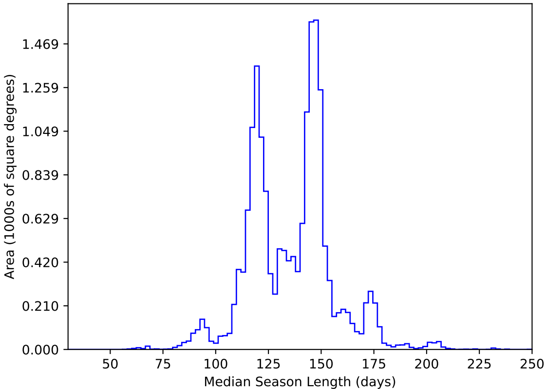
extra_ss_neo7_v3.4_10yrs WFD y band: Median Season Length
