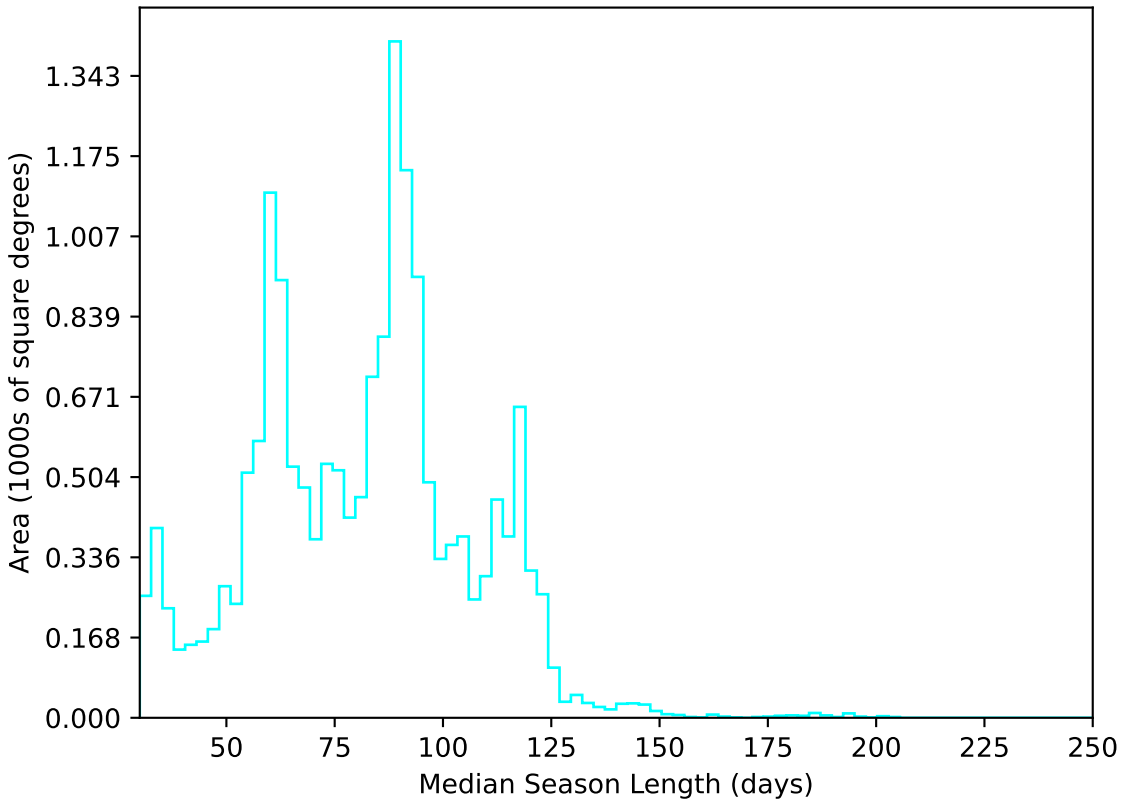
extra_ss_neo7_v3.4_10yrs WFD u band: Median Season Length
