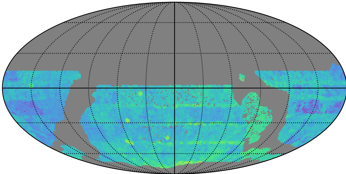
extra_ss_neo7_v3.4_10yrs WFD r band: Median Season Length
