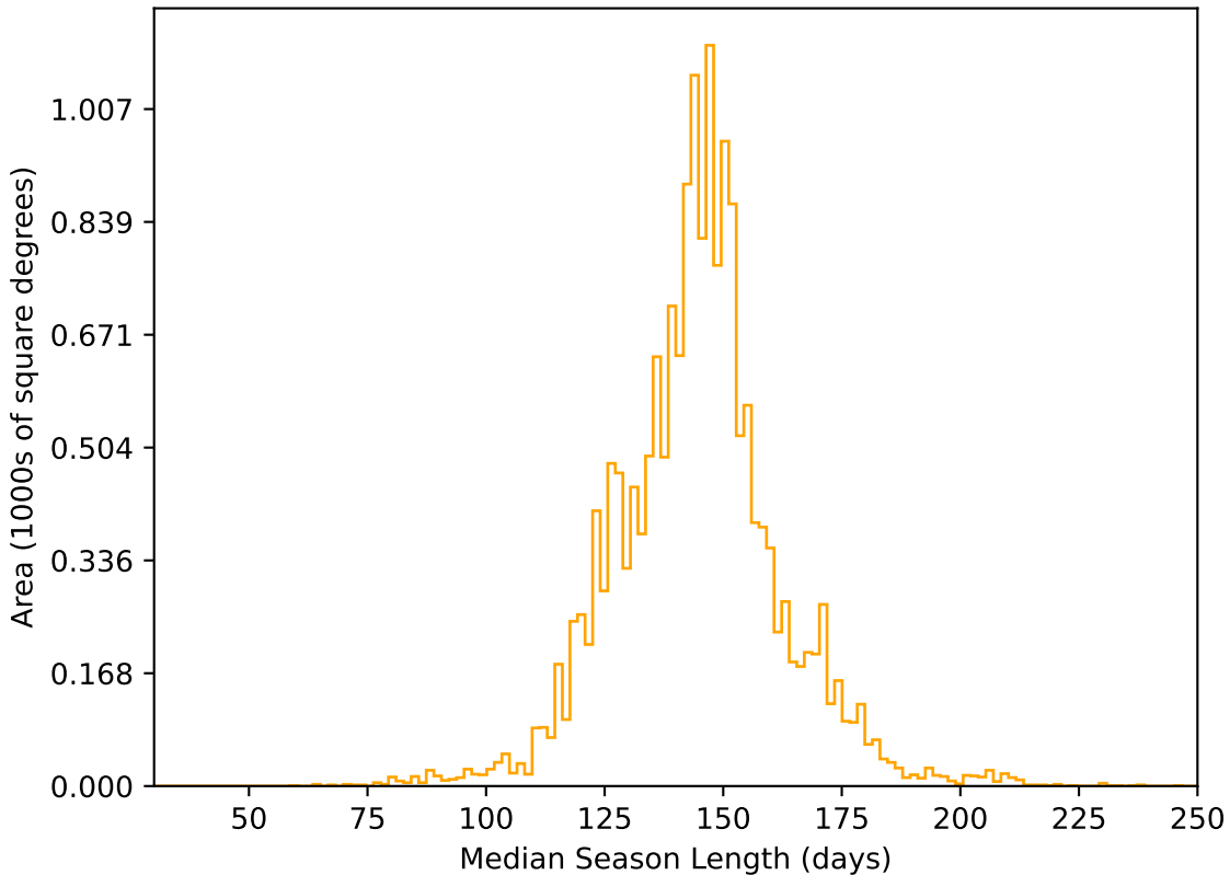
extra_ss_neo7_v3.4_10yrs WFD r band: Median Season Length
