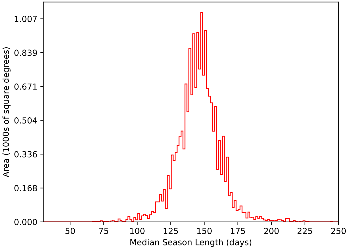
extra_ss_neo7_v3.4_10yrs WFD i band: Median Season Length
