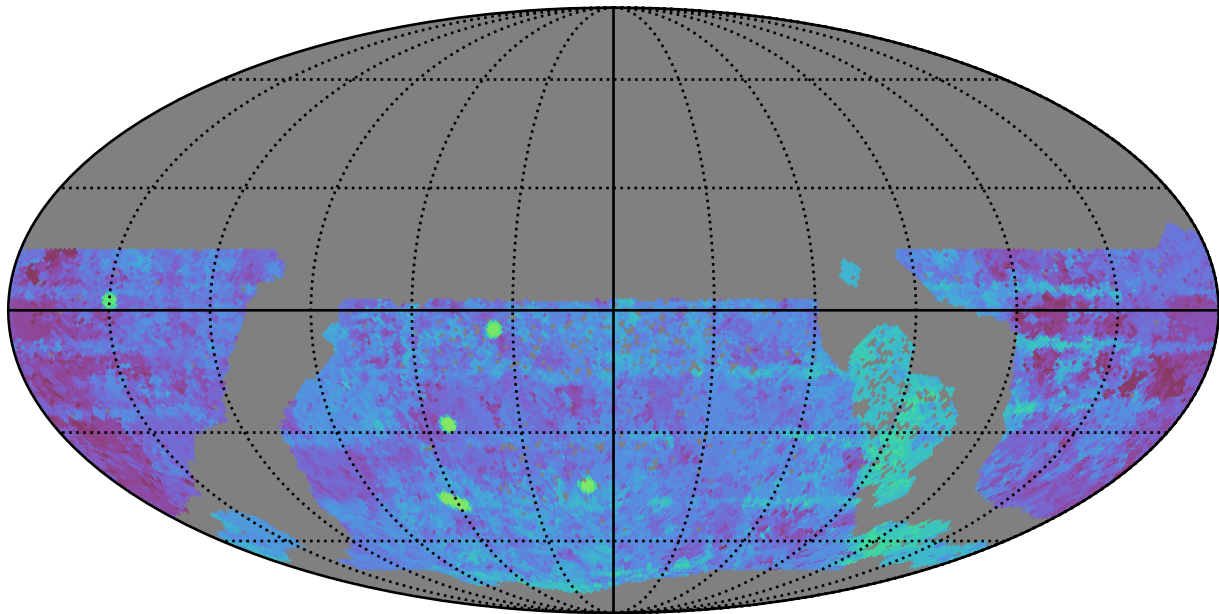
extra_ss_neo7_v3.4_10yrs WFD g band: Median Season Length
