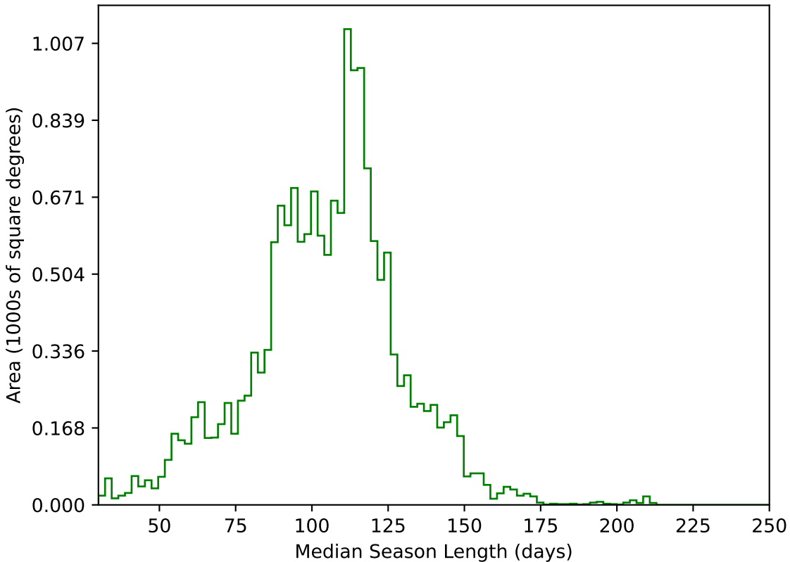
extra_ss_neo7_v3.4_10yrs WFD g band: Median Season Length
