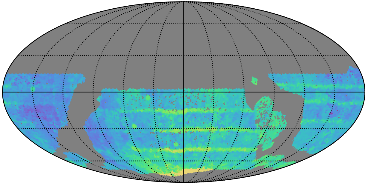
extra_ss_neo7_v3.4_10yrs WFD all bands: Median Season Length
