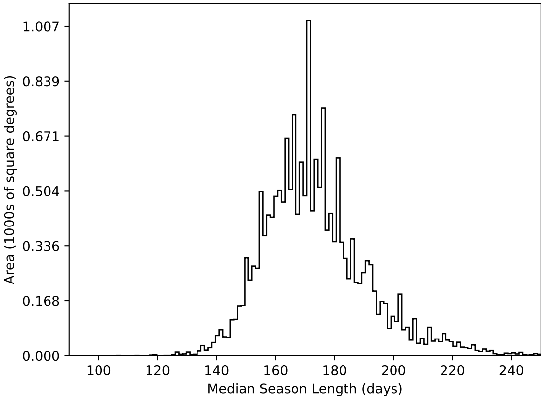
extra_ss_neo7_v3.4_10yrs WFD all bands: Median Season Length
