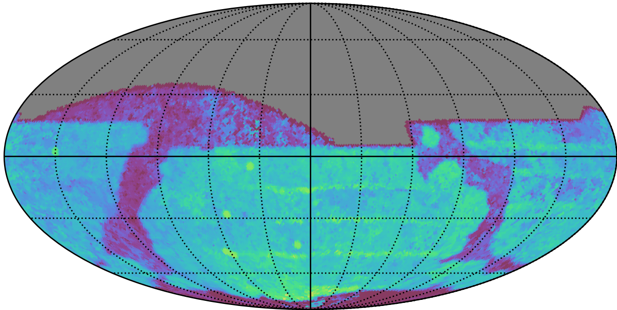
extra_ss_neo7_v3.4_10yrs All sky z band: Median Season Length
