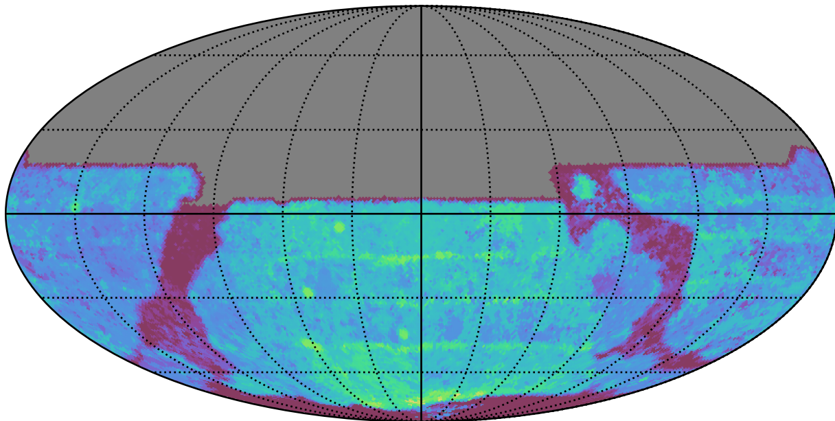
extra_ss_neo7_v3.4_10yrs All sky y band: Median Season Length
