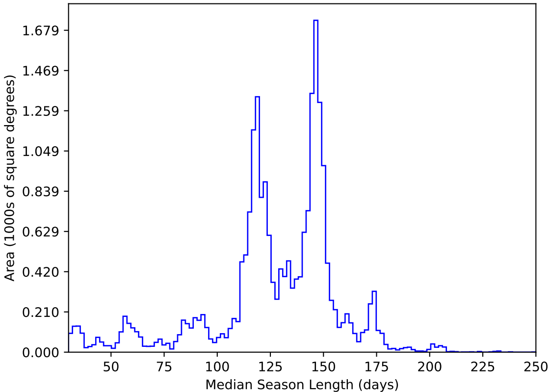
extra_ss_neo7_v3.4_10yrs All sky y band: Median Season Length
