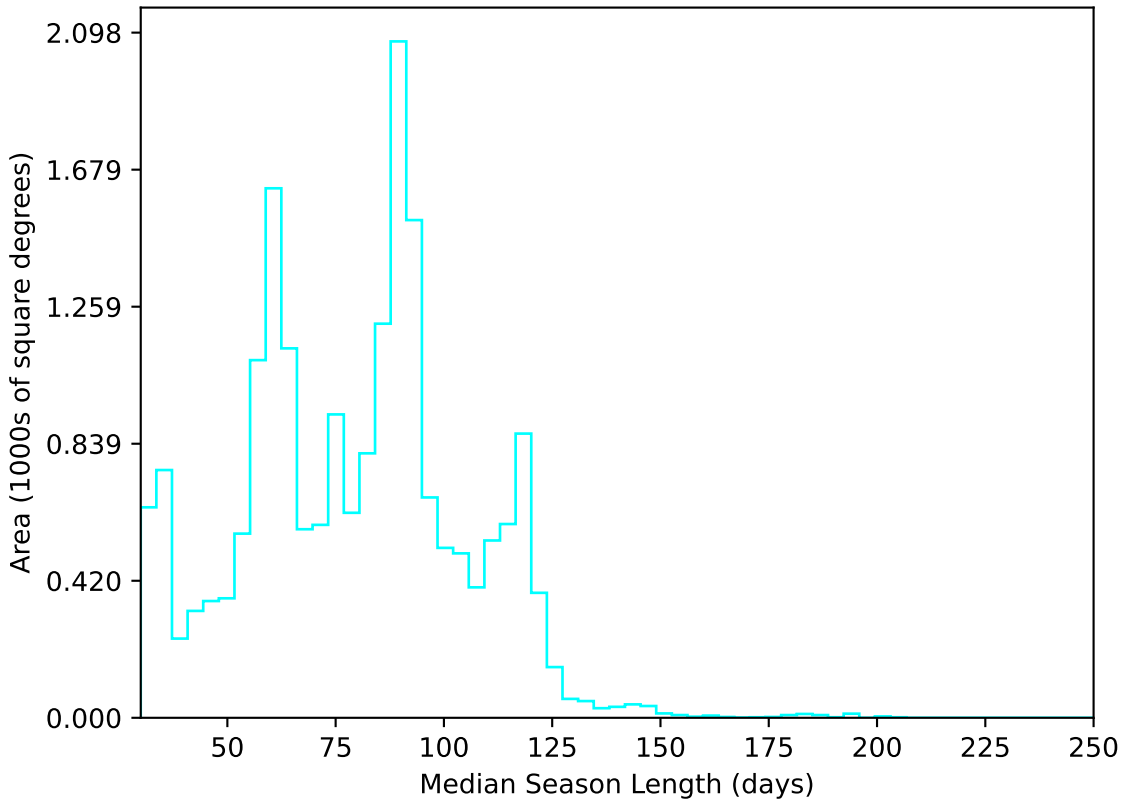
extra_ss_neo7_v3.4_10yrs All sky u band: Median Season Length
