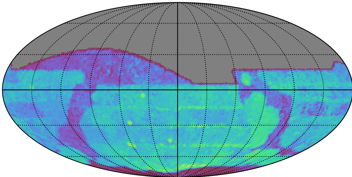
extra_ss_neo7_v3.4_10yrs All sky r band: Median Season Length
