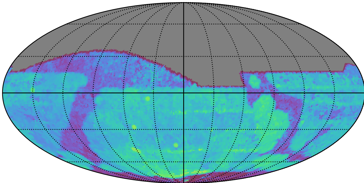
extra_ss_neo7_v3.4_10yrs All sky i band: Median Season Length
