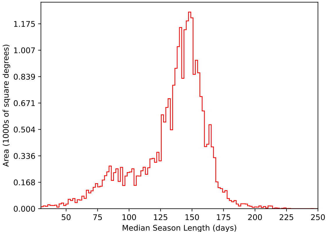
extra_ss_neo7_v3.4_10yrs All sky i band: Median Season Length
