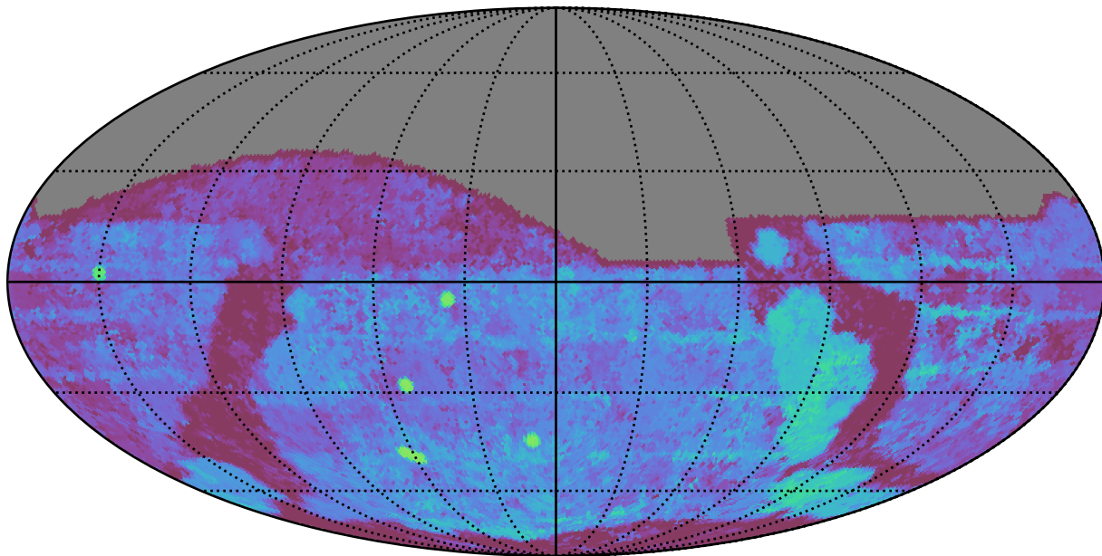
extra_ss_neo7_v3.4_10yrs All sky g band: Median Season Length
