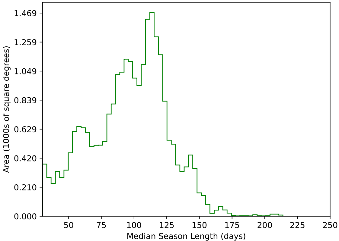
extra_ss_neo7_v3.4_10yrs All sky g band: Median Season Length
