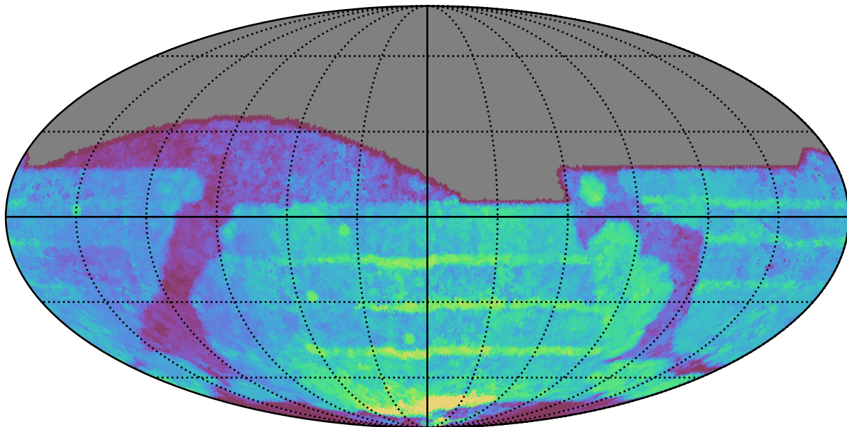
extra_ss_neo7_v3.4_10yrs All sky all bands: Median Season Length
