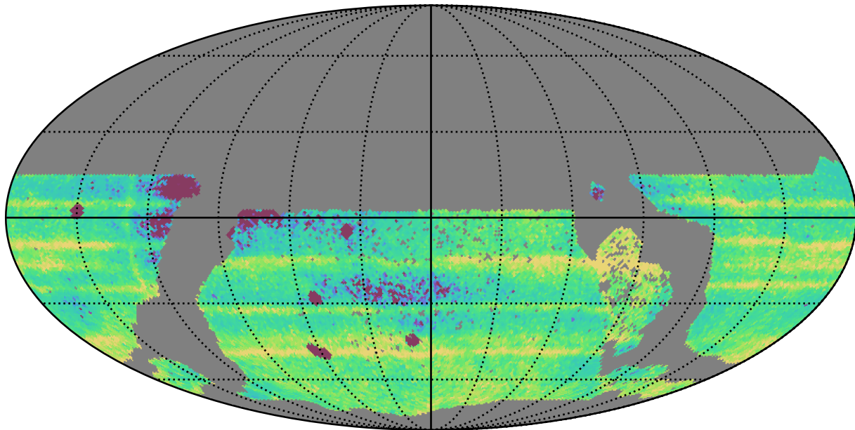
extra_ss_neo7_v3.4_10yrs WFD: Median Intra-Night Gap
