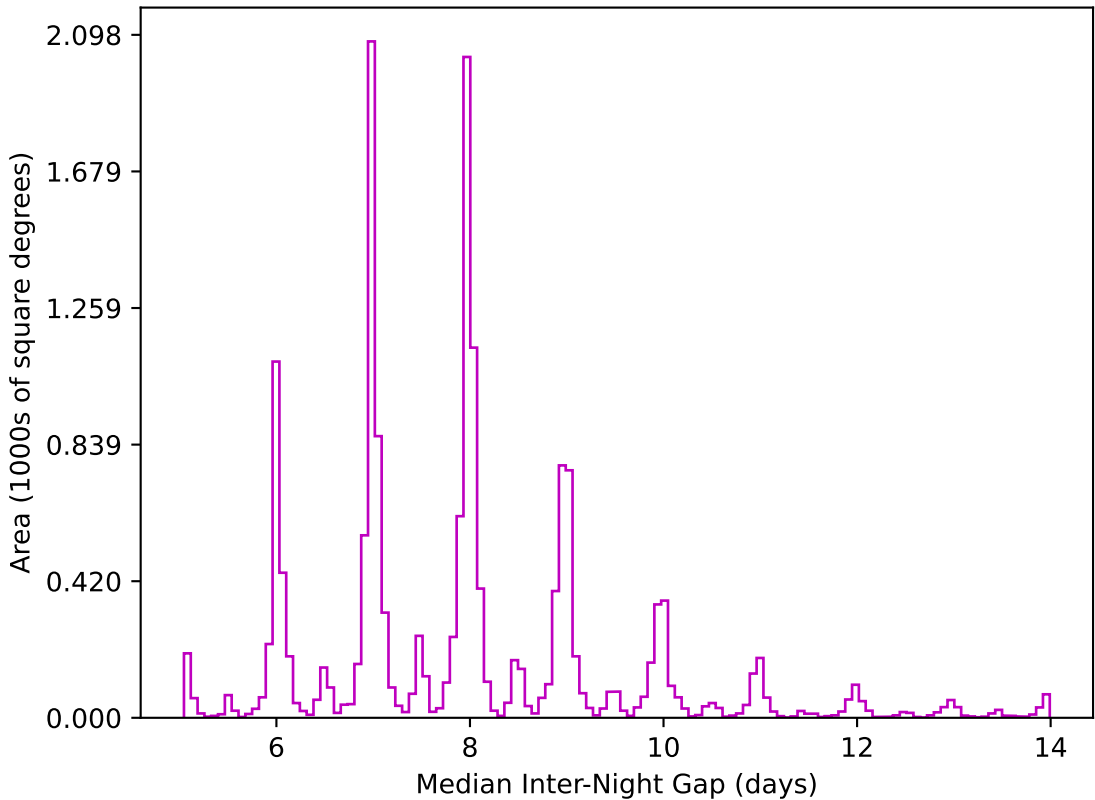
extra_ss_neo7_v3.4_10yrs WFD z band: Median Inter-Night Gap
