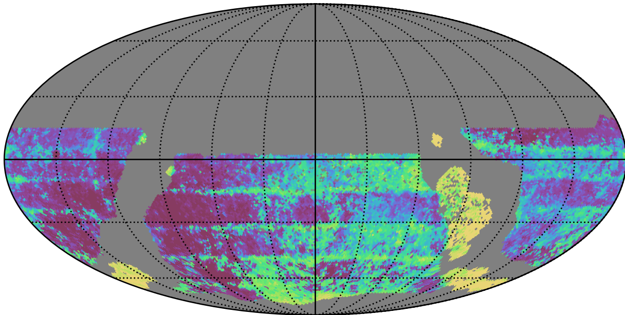
extra_ss_neo7_v3.4_10yrs WFD y band: Median Inter-Night Gap
