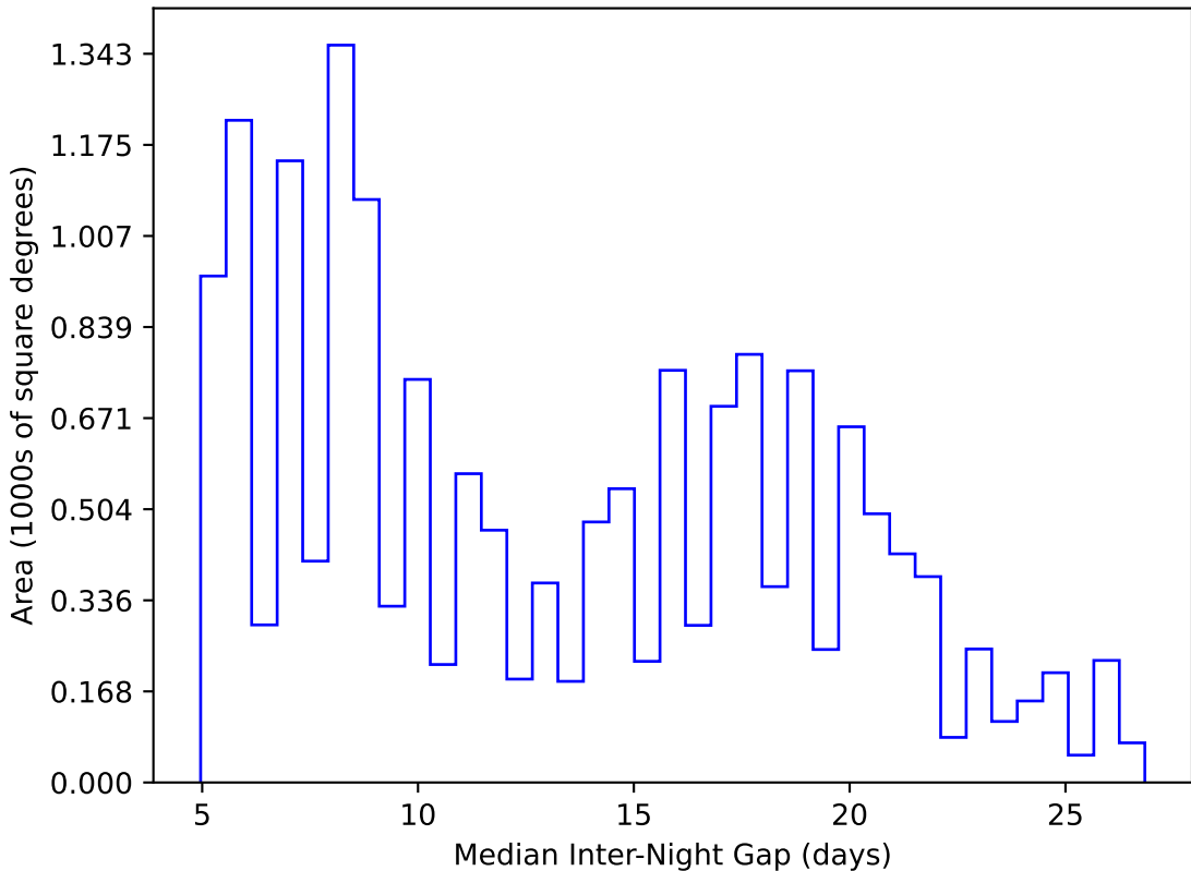
extra_ss_neo7_v3.4_10yrs WFD y band: Median Inter-Night Gap
