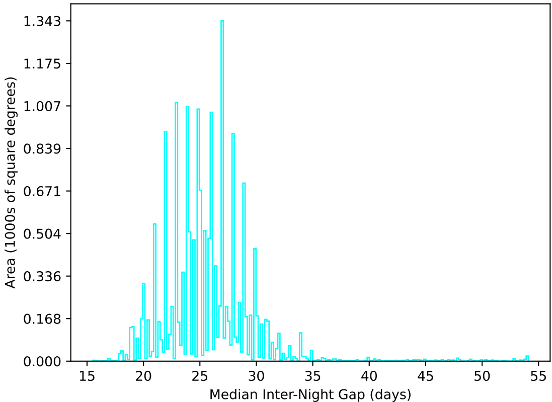
extra_ss_neo7_v3.4_10yrs WFD u band: Median Inter-Night Gap
