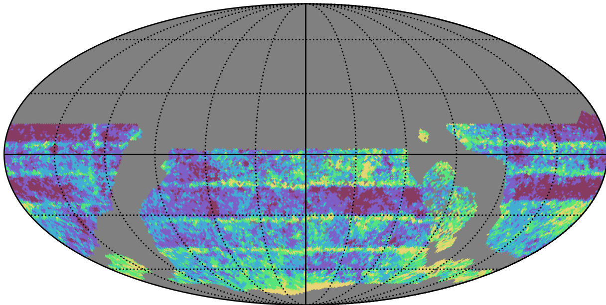
extra_ss_neo7_v3.4_10yrs WFD r band: Median Inter-Night Gap
