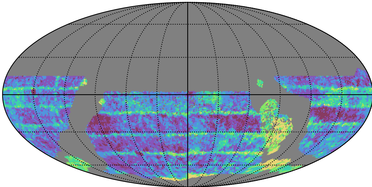
extra_ss_neo7_v3.4_10yrs WFD i band: Median Inter-Night Gap
