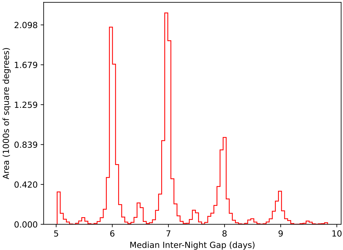
extra_ss_neo7_v3.4_10yrs WFD i band: Median Inter-Night Gap
