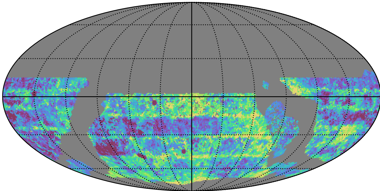
extra_ss_neo7_v3.4_10yrs WFD g band: Median Inter-Night Gap
