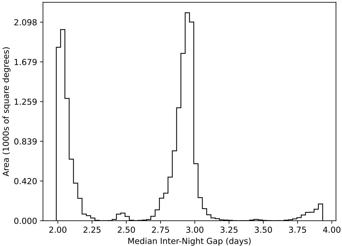
extra_ss_neo7_v3.4_10yrs WFD all bands: Median Inter-Night Gap
