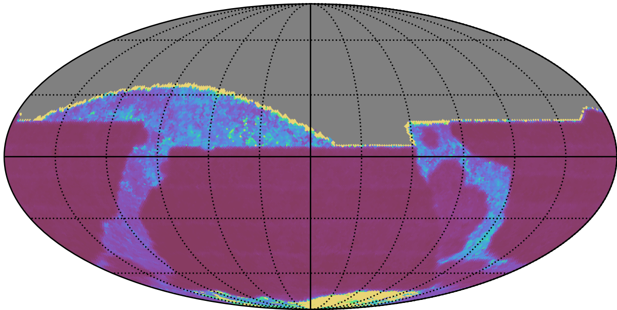
extra_ss_neo7_v3.4_10yrs All sky z band: Median Inter-Night Gap
