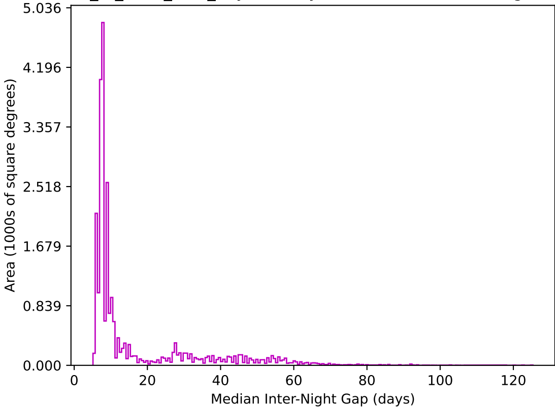
extra_ss_neo7_v3.4_10yrs All sky z band: Median Inter-Night Gap
