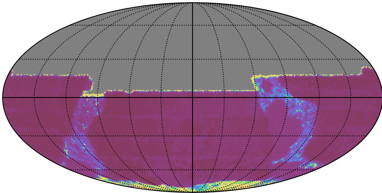
extra_ss_neo7_v3.4_10yrs All sky y band: Median Inter-Night Gap
