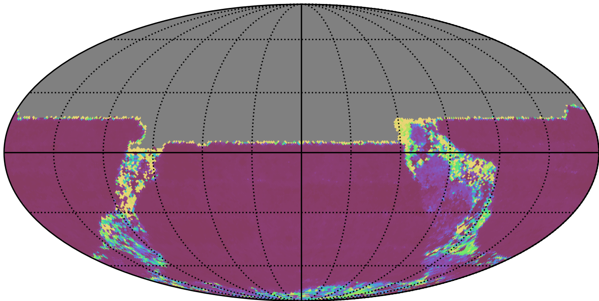
extra_ss_neo7_v3.4_10yrs All sky u band: Median Inter-Night Gap
