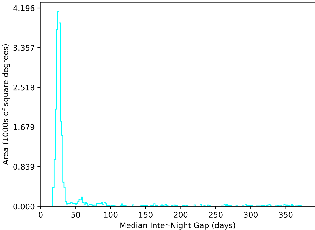
extra_ss_neo7_v3.4_10yrs All sky u band: Median Inter-Night Gap
