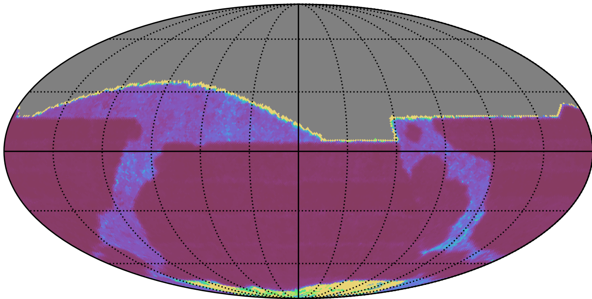
extra_ss_neo7_v3.4_10yrs All sky r band: Median Inter-Night Gap
