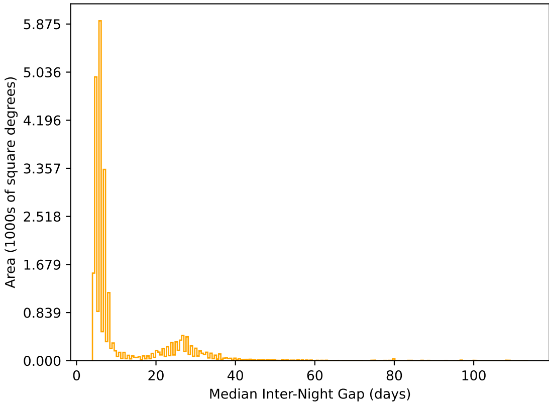
extra_ss_neo7_v3.4_10yrs All sky r band: Median Inter-Night Gap
