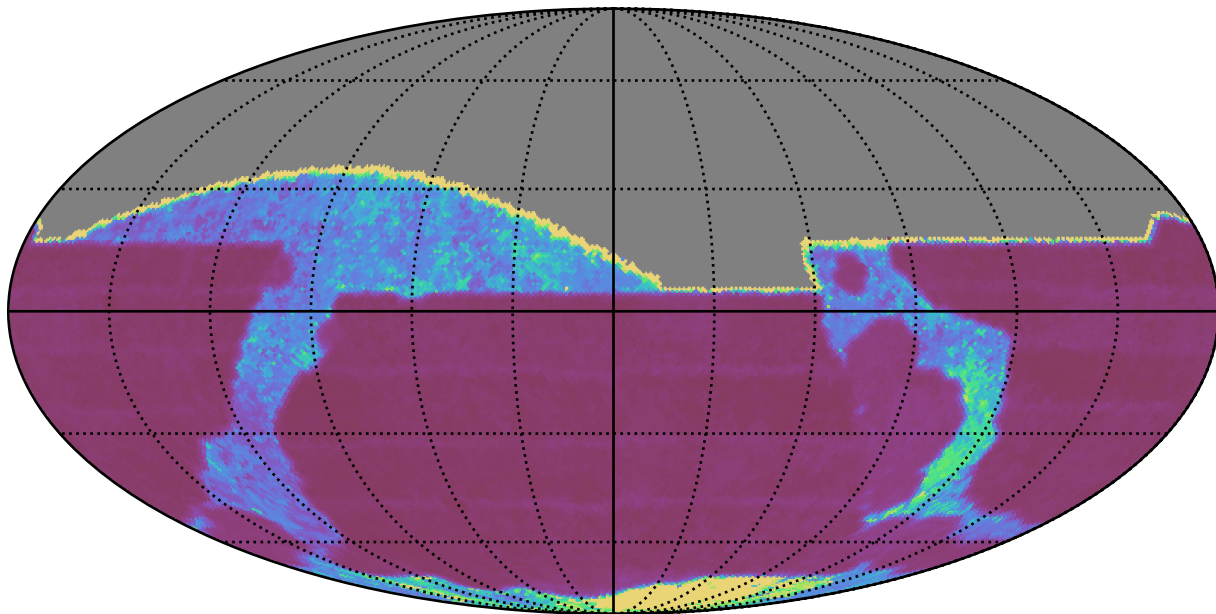
extra_ss_neo7_v3.4_10yrs All sky i band: Median Inter-Night Gap
