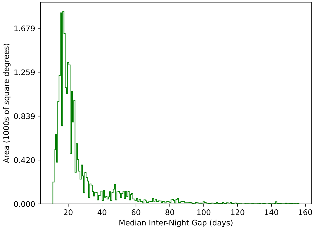
extra_ss_neo7_v3.4_10yrs All sky g band: Median Inter-Night Gap
