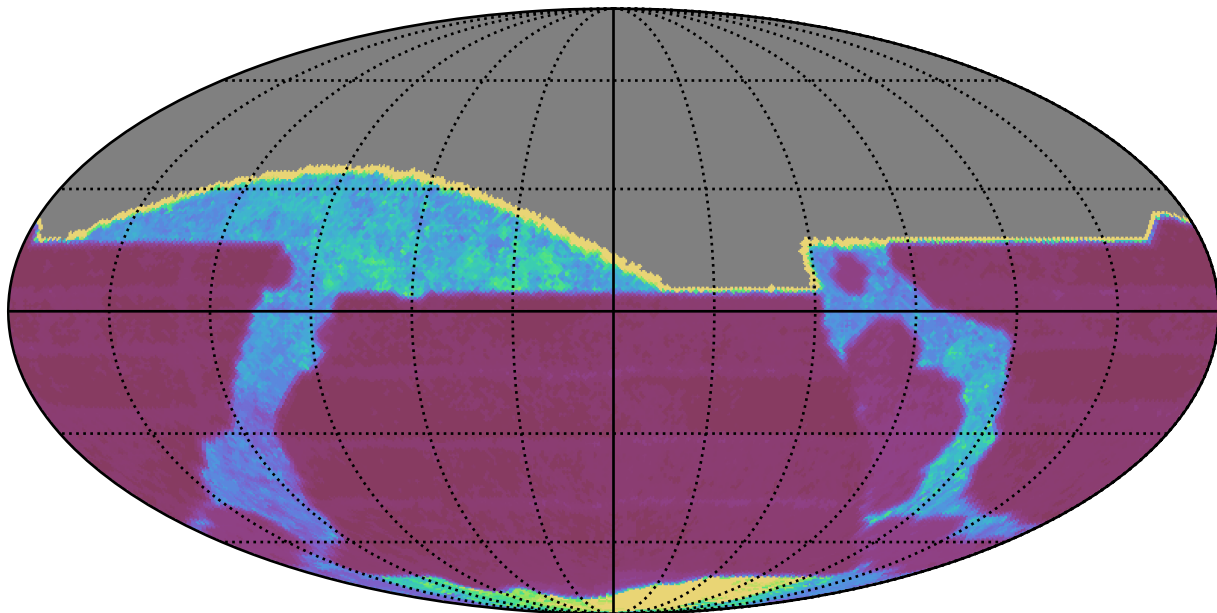
extra_ss_neo7_v3.4_10yrs All sky all bands: Median Inter-Night Gap
