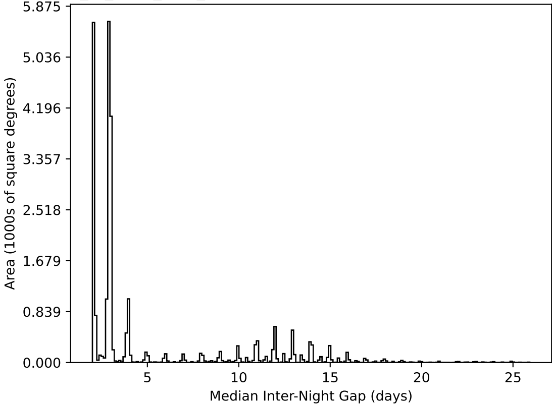
extra_ss_neo7_v3.4_10yrs All sky all bands: Median Inter-Night Gap
