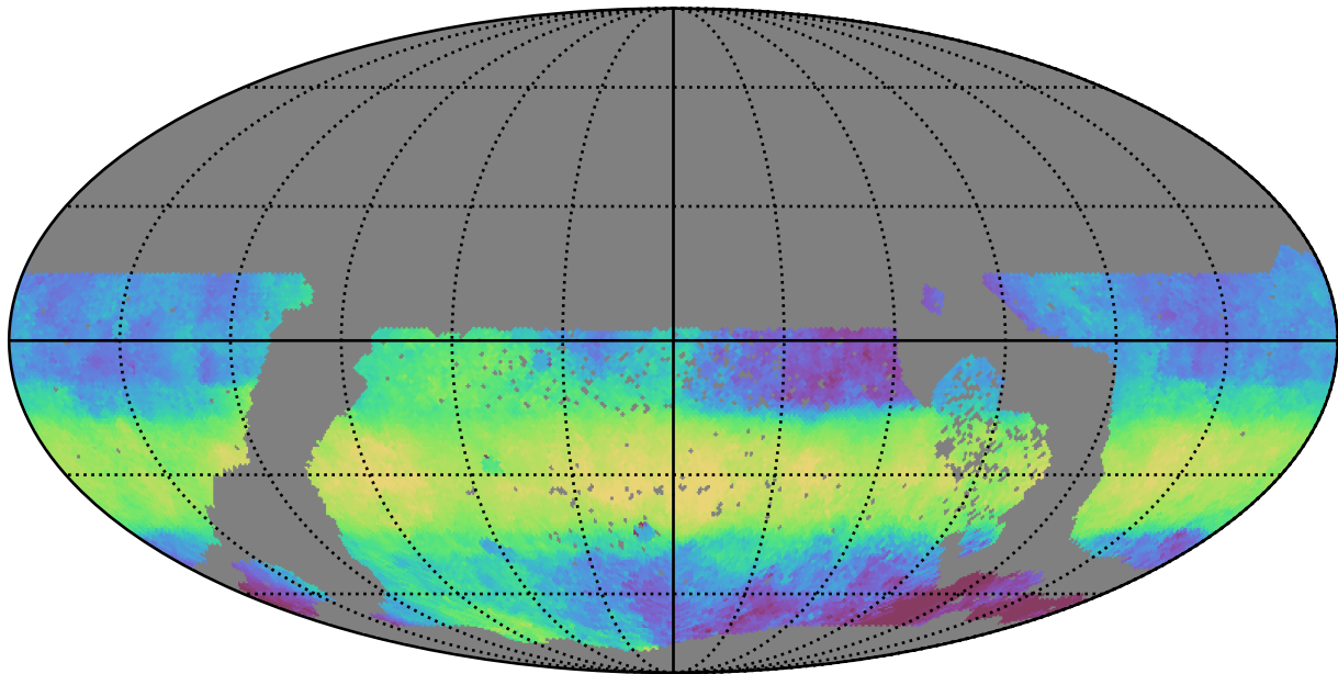
extra_ss_neo7_v3.4_10yrs WFD z band: Median HA
