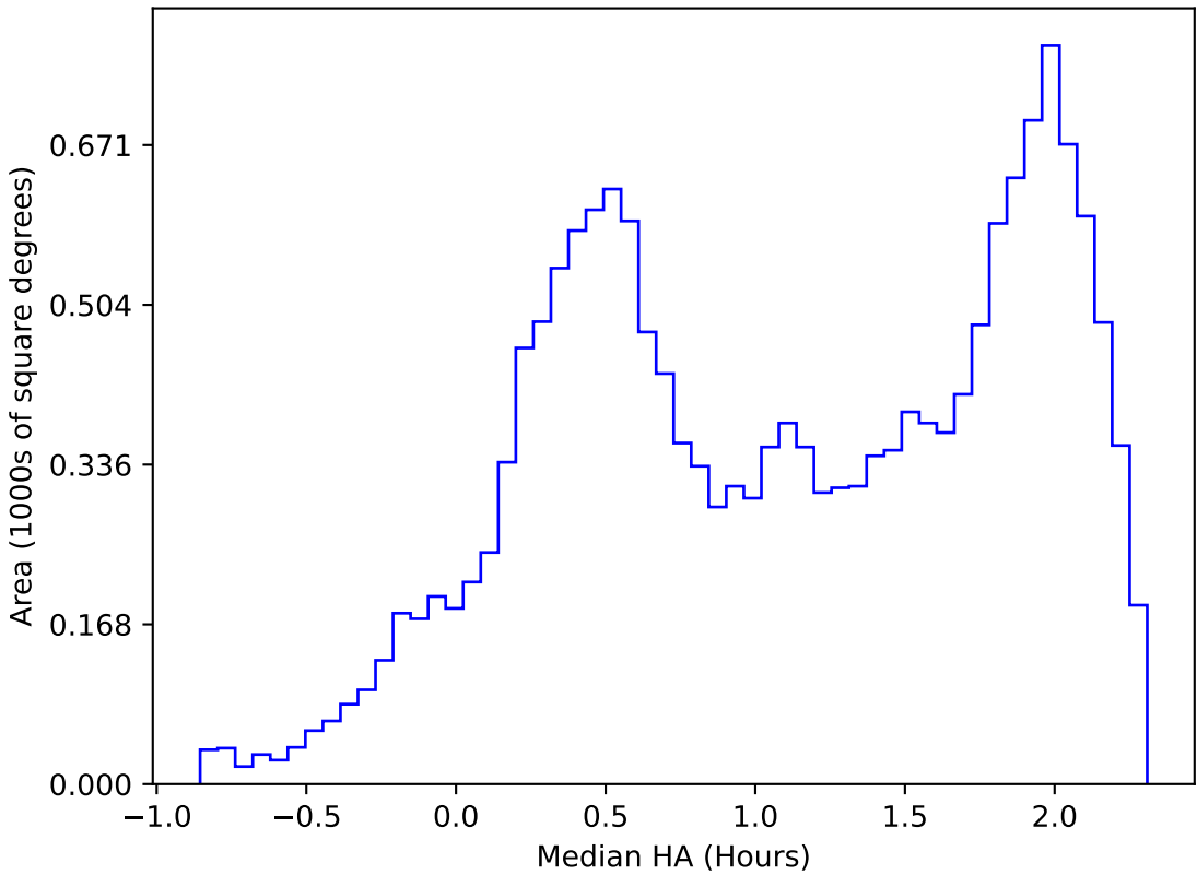
extra_ss_neo7_v3.4_10yrs WFD z band: Median HA
