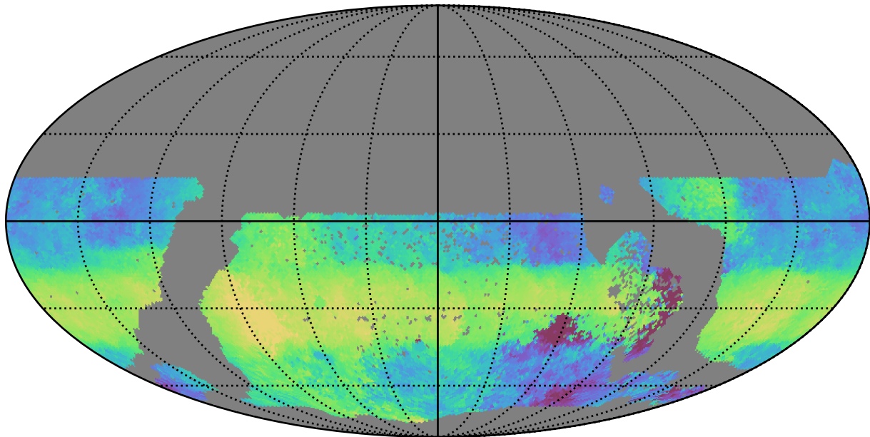
extra_ss_neo7_v3.4_10yrs WFD u band: Median HA
